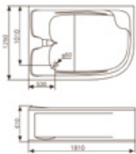
G9027(Left) Left Skirt Panel: you will see the bathtub installed against a LEFT corner of the wall when you face to it.
