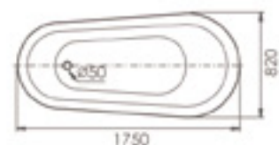
size:1750x820x820mm G9030-D
