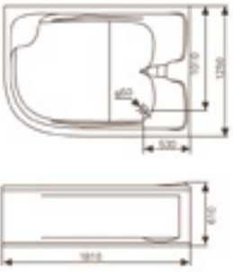
G9027(Right) Right Skirt Panel: you will see the bathtub installed against a RIGHT corner of the wall when you face to it.
