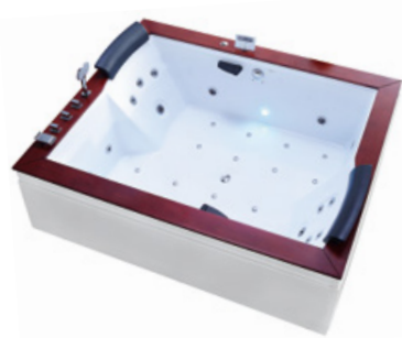
G9052-II Size:1860x1510x820mm
